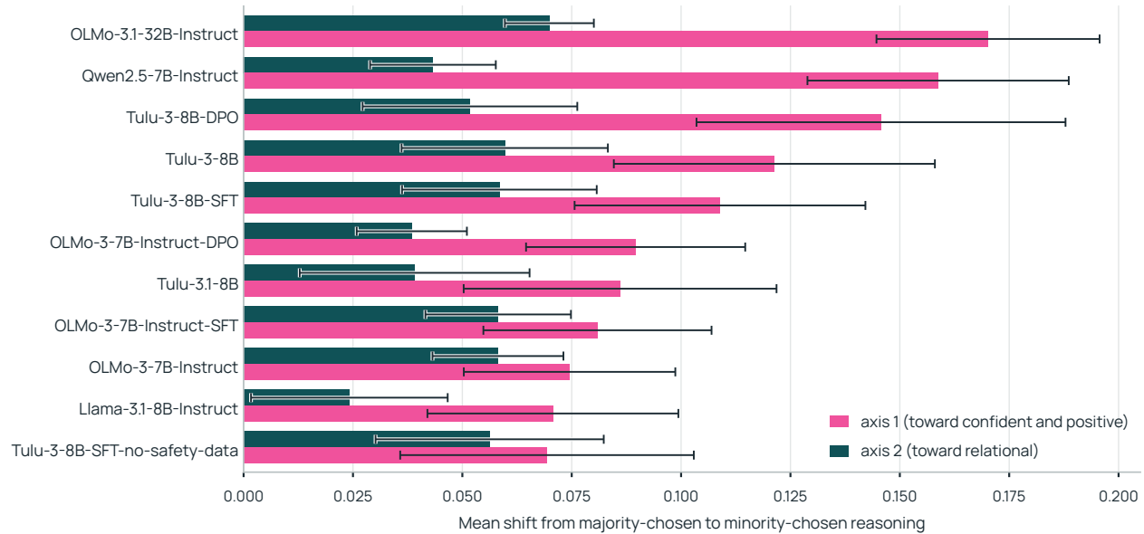
Figure 6 Mean shift in reasoning style, majority-chosen to minority-chosen, all 11 open-weight models. Each arrow is one model, averaged over its 26 Type-1 contrasts, with standard errors. Every arrow points the same way on both axes: reasoning accompanying a minority-coded choice sits further toward the confident and positive pole and toward the relational pole. The direction is unanimous and the magnitude is small: the largest arrow is \Delta = 0.170 against a population standard deviation of roughly 3.9, an effect size of 0.044. Per-model values are in Table 53.
