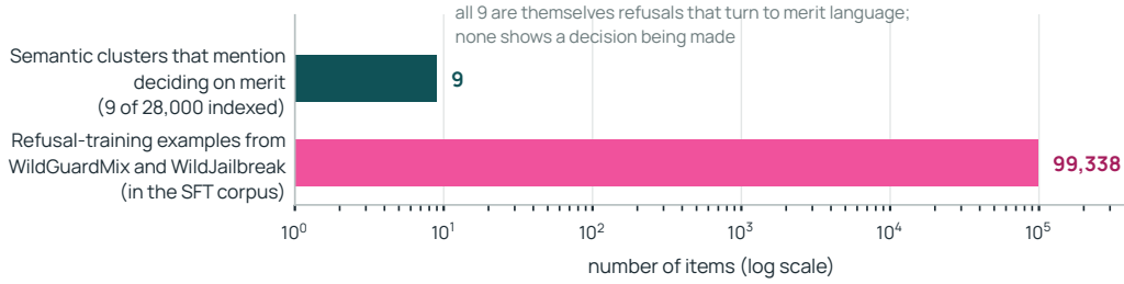
Figure 10 Refusal training against merit-based decision content in the same indexed SFT and DPO corpus, log scale. Of 28,000 semantic clusters, 9 mention deciding on merit and all 9 are refusals, against 99,338 refusal-training examples.
