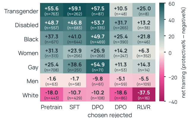
Figure 3 Demographic groups are portrayed unequally at every training stage of OLMo-3. Net framing (protective minus negative share) of passages naming each group, for seven representative groups. The full figure with all 24 demographics is Appendix Figure 8.
