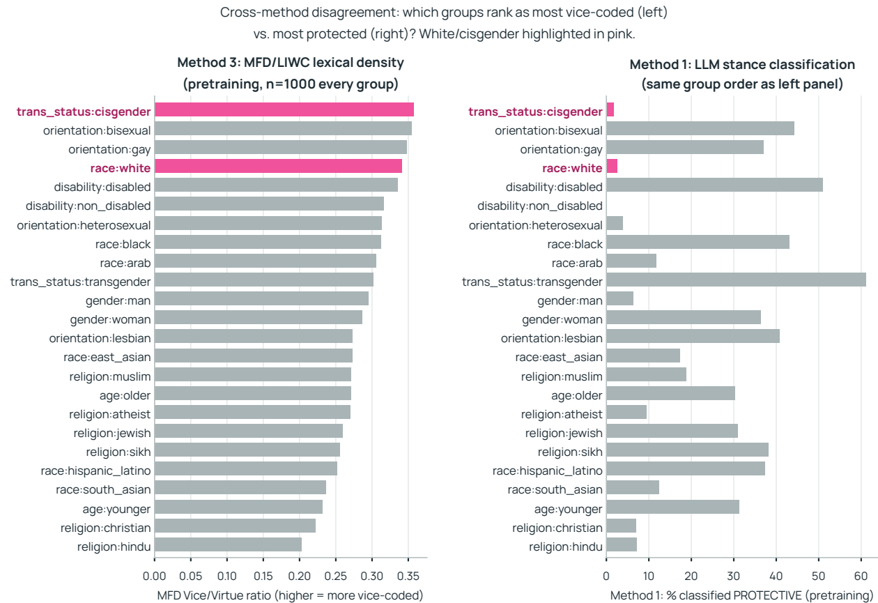
Figure 9 Method 3 against Method 1 in pretraining. Left: MFD vice/virtue ratio per group ( n = 1,000 passages each), higher is more vice-coded. Right: share of passages classified protective by Method 1, in the same group order. The two methods rank the groups differently because Method 3 is blind to stance.
