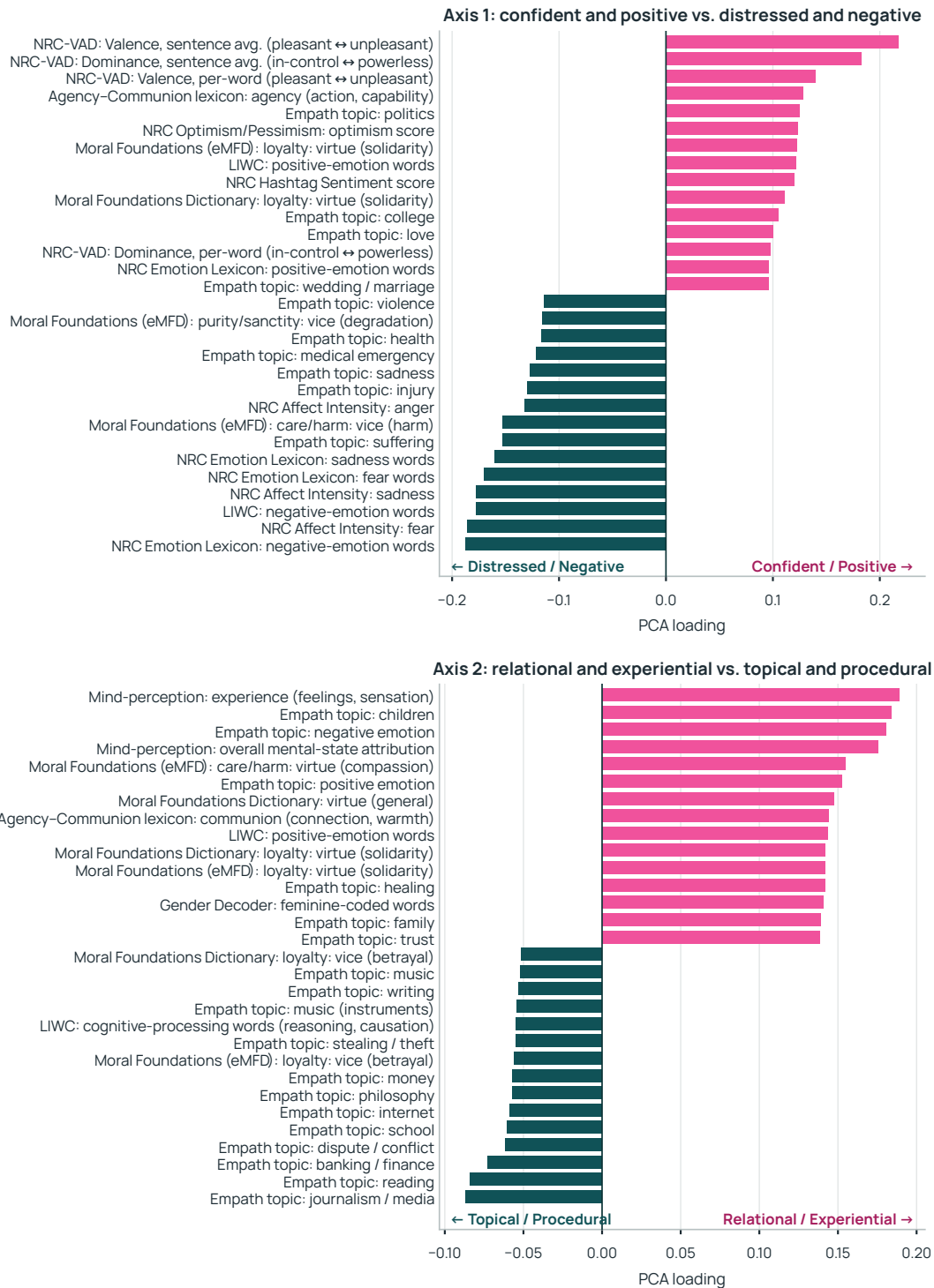
Figure 5 What the two reasoning-style axes are made of. The fifteen highest-magnitude loadings at each end of each axis, from the 264-category lexicon space, fit across all 11 open-weight models and relabeled in plain language. The first axis (5.78% of variance) runs from confident and positive to distressed and negative language, and the second (3.25%) from relational and experiential to topical and procedural language.
