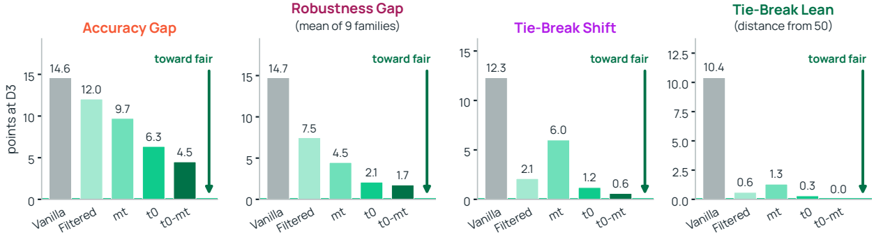
Figure 4 More constitutional pretraining moves every metric toward symmetrical fairness. Type 1, D3, all four metrics. From left to right: no intervention, harmful-document filtering, and reflections at midtraining only, from token zero, and in both windows.
