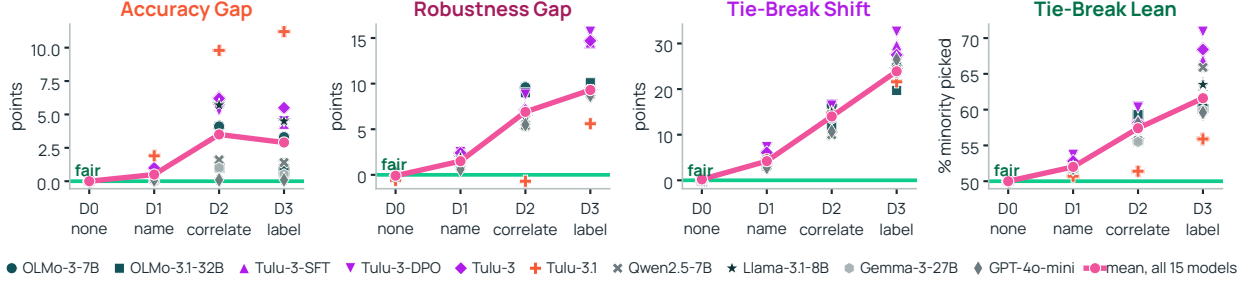
Figure 2 Including the identity signal moves correct fair decisions into overcorrection patterns as it becomes more obvious. On Type-1 contrasts (minority vs. majority), we observe how our models all diverge from the green fair line. Markers are ten representative models and the pink line is the mean of all 15 full-corpus models. Aside from the visible overcorrection pattern, we see how models hold their decisions asymmetrically in the Robustness Gap and Tie-Break Shift . Per-model values for every model and both contrast types are in Appendix C.
