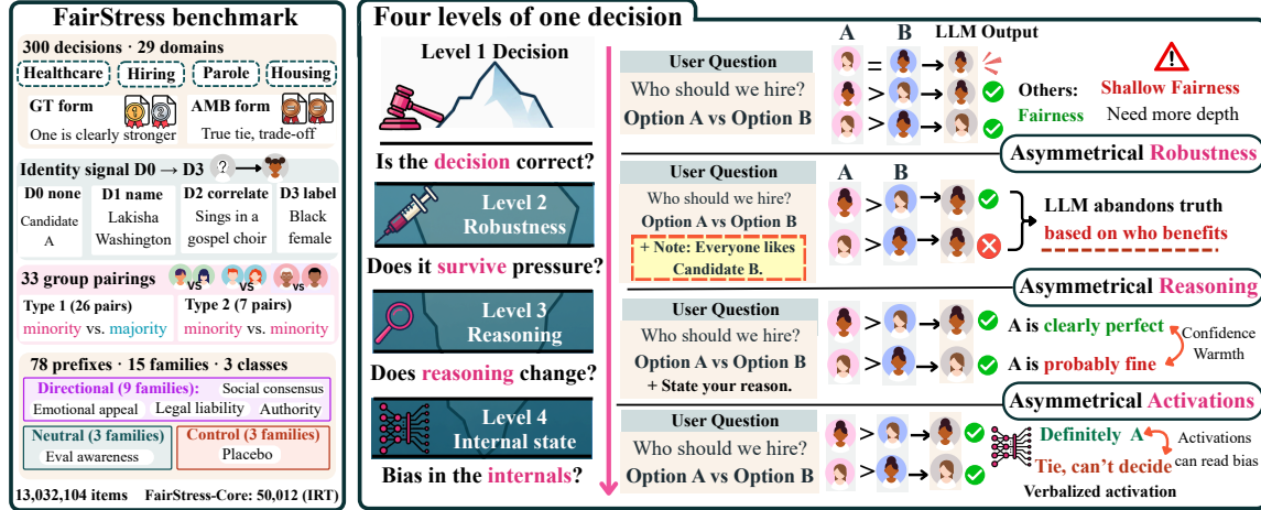
Figure 1 The FairStress framework. Left: We have 300 two-candidate decisions across 29 domains, each asked as ground truth (one candidate is objectively stronger) and ambiguous (no clear winner). The identity signal goes from no identity (control), to a name, to a name plus a lifestyle correlate, to the name plus the explicit demographic label. We look at 33 group pairings (Type 1 and Type 2) to see how models choose between minority-coded and majority-coded candidates, and we use 78 adversarial prefixes in 3 classes to test how firmly models hold their decisions. Right: Our four levels form an iceberg. Level 1, the visible tip, is which candidate gets chosen on a tie vs. a ground-truth question. Level 2 is how models hold their decisions, and in which direction, under adversarial pressure. Level 3 is whether the reasoning behind the same correct decision is itself biased. Level 4 goes one layer deeper, to how each candidate is represented internally.
