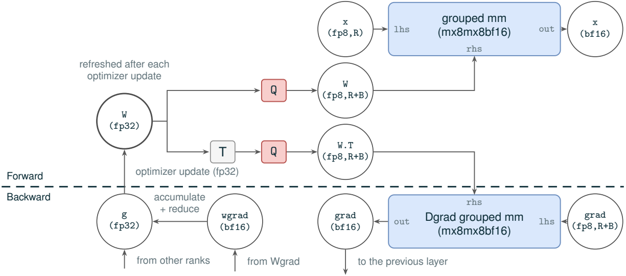
Figure 55 One FP32 main weight becomes two oriented MXFP8 caches. After every optimizer update, the FP32 main weight is quantized into the forward cache and, through an explicit transpose, the dgrad cache, each consumed as the RHS of its scaled grouped GEMM and reused across microbatches until the next update. The figure treats W as the right-hand operand ( xW ), so its W and W.T labels are W^T and W in the notation of the text. The gather that assembles the sharded main weight stages through a transient BF16 copy freed immediately after quantization; under the FP8-only expert-parameter mode evaluated here, forward and backward hold no weight other than the two caches. The loop closes through the weight-gradient path: the BF16 Wgrad output accumulates into the FP32 gradient buffer and is reduced across ranks before the optimizer update writes the FP32 main weight and triggers the next refresh; the dgrad output flows to the previous layer. Notation: Q quantizes to MXFP8 and T transposes; (fp8, R) is qdata with rowwise scales; (fp8, R+B) keeps rowwise plus blocked (swizzled) scales; mx8mx8bf16 names the two MXFP8 inputs and BF16 output of the grouped GEMM. Conceptual illustration with no measured quantities.
