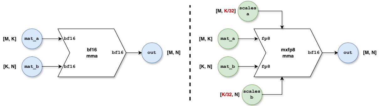
Figure 47 BF16 and native MXFP8 Tensor Core paths. For A \in \mathbb{R}^{M \times K} and B \in \mathbb{R}^{K \times N} , the MXFP8 operation consumes E4M3 qdata and logical scale grids of shape M \times (K/32) and (K/32) \times N before scale swizzling. “MMA” names the native Tensor Core operation accurately: Blackwell provides tcgen05.mma instructions with the kind:mx8f6f4 and block_scale modifiers for this computation. Olmo invokes the higher-level scaled_mm operator, whose kernel includes the MMA main loop and an epilogue that converts the accumulator to the requested BF16 output. Thus, BF16 labels the completed operator output, not the raw MMA accumulator.
