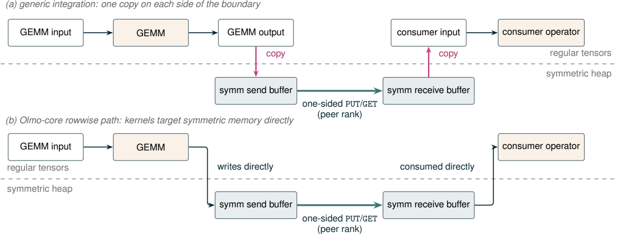
Figure 20 Crossing the regular-symmetric boundary: staging copies versus direct access. The remote endpoint of a one-sided transfer must live in the symmetric heap, which is allocated separately from regular PyTorch tensors; inter-node GPU-initiated transfers require the local endpoint to be symmetric as well. (a) A generic integration pays one copy on each side of the boundary. (b) The Olmo-core rowwise path removes these copies where kernels can target symmetric memory directly: the expert grouped GEMM reads the dispatch buffer in place, the down projection writes its output directly into the symmetric combine buffer, and MXFP8 dispatch fuses quantization into the PUT kernel. Conceptual illustration with no measured quantities.
