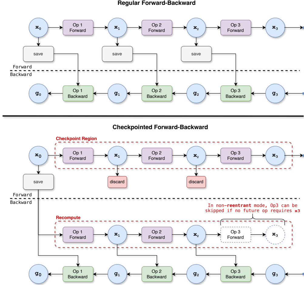
Figure 61 Non-reentrant checkpointing can stop recomputation early. A regular forward saves the intermediate values required by each backward operator. A checkpointed forward instead retains the region input x_0 and discards x_1 and x_2 . During backward, the region is recomputed until those required values have been regenerated. In this simplified example, Op 3’s forward need not be recomputed because Op 3 backward requires x_2 , while the original checkpoint output x_3 remains available to downstream computation. The general stopping condition is determined by backward’s tensor requirements, not merely by the position of an operator in the region.
