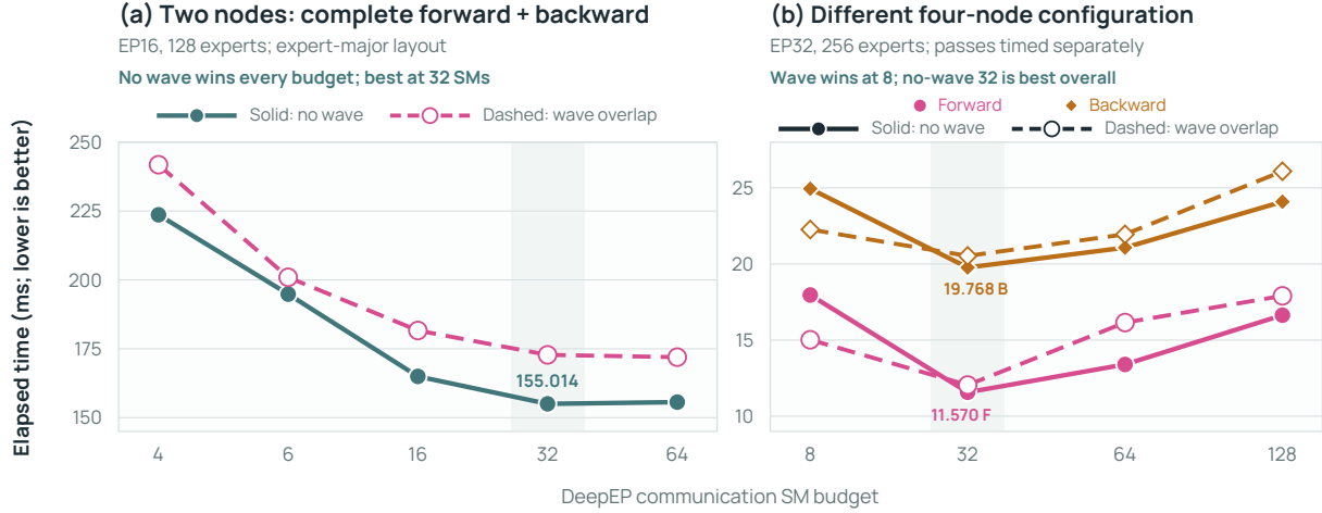
Figure 24 No-wave execution is fastest after tuning the communication-SM budget in both sweeps. The panels show absolute elapsed time with independent vertical scales; lower is better. (a) On the two-node EP-MP = 16, 128-expert, expert-major BF16 configuration, no-wave was faster at every communication-SM budget and reached its minimum at 32 SMs. (b) On a different four-node EP-MP = 32, 256-expert, source-token-major BF16 configuration, overlap beat no-wave at the communication-constrained eight-SM point. Nevertheless, no-wave at 32 SMs remained the best measured forward and backward operating point. Panel (a) reports max-rank medians over five iterations after 10 warm-ups with inter-iteration synchronization; panel (b) reports max-rank medians over five iterations after three warm-ups without that synchronization. Both are Nsight-instrumented standalone development runs.
