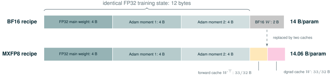
Figure 48 Persistent memory with BF16 weights and two MXFP8 weight caches. Nominal bytes per parameter: both recipes keep the FP32 main weight and two FP32 Adam moments; the BF16 recipe adds one two-byte compute weight, while the MXFP8 recipe replaces it with the forward and dgrad weight caches at 33/32 bytes each. Gradient buffers are identical in both recipes and excluded, and blocked-scale padding is ignored. Conceptual illustration of the nominal accounting with no measured quantities.
