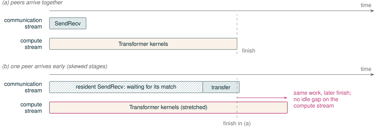
Figure 27 A resident P2P wait can slow the compute meant to hide it. With matched arrival (a), the send/receive kernel transfers and exits, and the overlapped Transformer kernels run at full speed. With skewed arrival (b), the early peer’s resident send/receive kernel occupies streaming multiprocessors while it waits for its match, so the overlapped compute stretches even though no idle gap appears on the compute stream. Conceptual illustration with no measured quantities.
