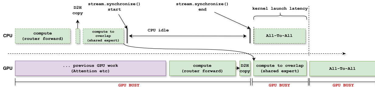
Figure 34 Independent compute can cover a host wait without removing it. The CPU submits shared-expert work before blocking on GPU-produced route counts, so the GPU remains busy while the host waits. The all-to-all still cannot be submitted until the counts are host-visible. This is latency coverage, not communication-compute overlap; the timeline is conceptual and does not encode measured duration.
