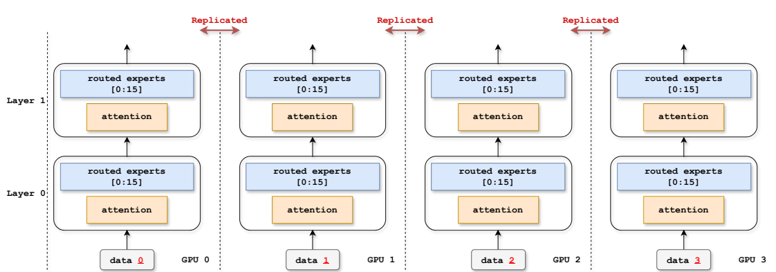
Figure 6 A four-GPU DDP example with no model-parallel sharding. With DP = 4 , every GPU holds a static replica of the same attention layers and complete routed-expert pool, experts 0–15, while processing different input data. DDP synchronizes the gradients of these replicated weights; it does not itself shard the model shown here.
