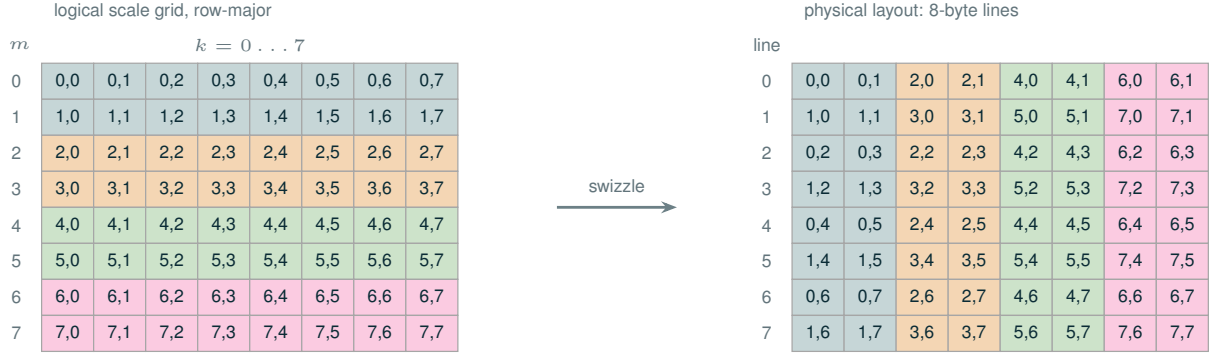
Figure 52 The scale order a GEMM consumes is a tiled, interleaved layout. Cells are labeled m, k for the scale of row m and block column k , and colors mark row groups. Before the swizzle the grid is row-major; after it, each physical line interleaves the four row groups while a row’s scales within a tile stay adjacent. The drawing is a structure-preserving miniature with two-row groups and two-column tiles; the hardware layout applies the same rule with 32-row groups and four-column tiles, rearranging 128 \times 4 tiles of scales into 32 sixteen-byte lines so that rows m , m+32 , m+64 , and m+96 become physically adjacent (NVIDIA, 2026p). The result resembles a transpose because whole row-group sub-blocks are relocated from a vertical stack to a horizontal line, but it is not one: inside every sub-block, m still advances downward and k rightward, and each scale keeps its m, k identity; only its address changes. Conceptual illustration with no measured quantities.
