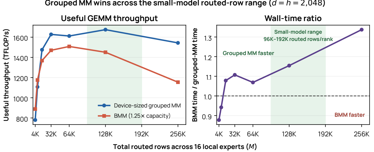
Figure 71 Grouped GEMM also wins across the small-model training range. This one-B300 experiment fixes 16 local experts and a square BF16 projection with d = h = 2048 . The green band marks the 96K–192K routed-row range represented by the small configurations in Table 42; their exact widths and local expert counts vary, so the band is an operating-range guide rather than an exact reconstruction of every model. BMM reserves 1.25\times capacity per expert, while grouped GEMM executes only valid rows. Each point averages 20 queued CUDA-event samples after 10 warm-ups.
