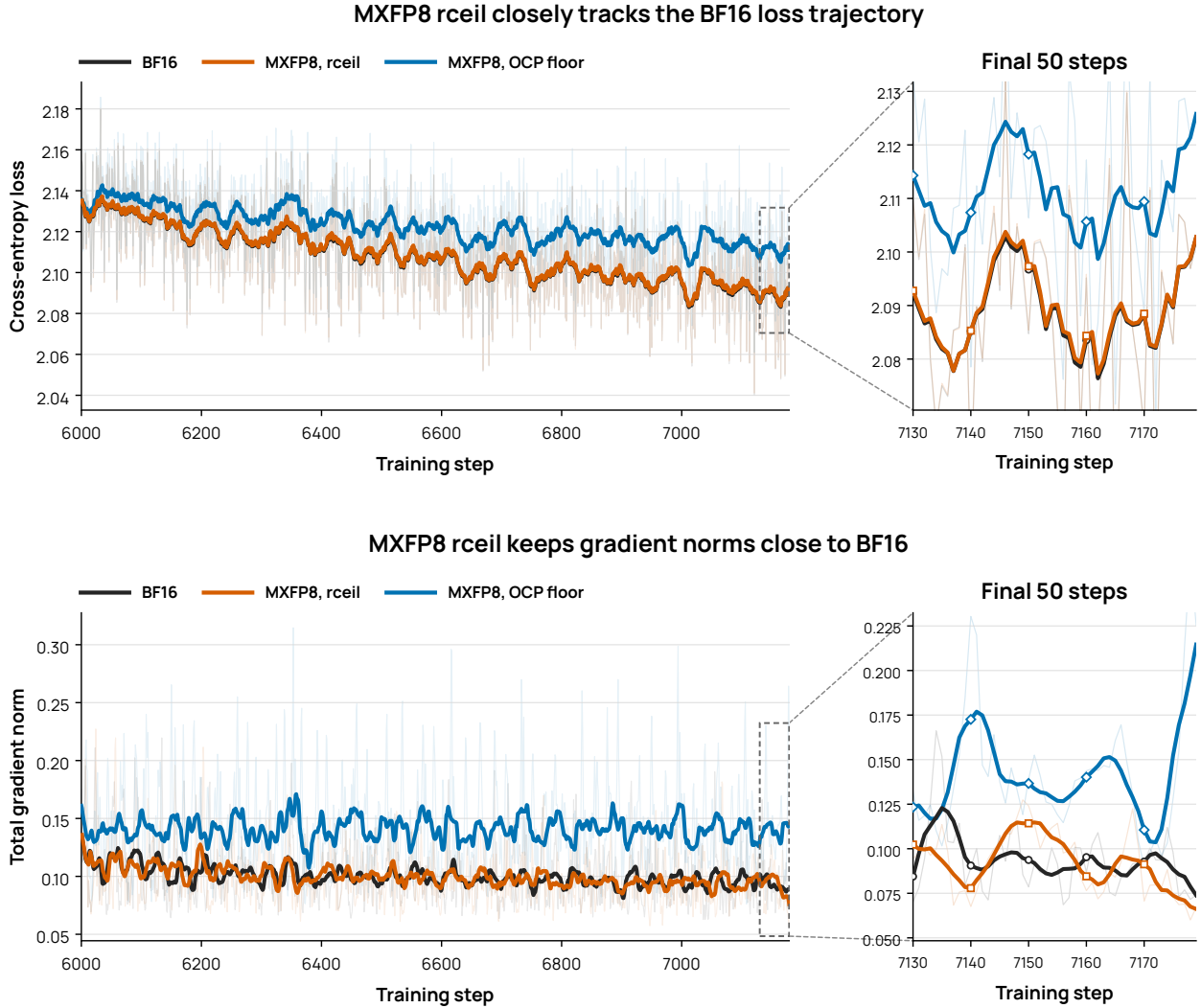
Figure 56 Round-ceiling MXFP8 follows the BF16 training trajectory. The top plot reports cross-entropy loss; the bottom reports total gradient norm. The model has 8.36B active and 166.72B total parameters across 31 layers, with top-4 routing over 128 routed experts and one shared expert. The common step-6000 checkpoint was trained from scratch with MXFP8 OCP-floor scaling on approximately 56B tokens. Step 7179 corresponds to approximately 67B tokens, so the plotted continuation spans approximately 11B tokens. The main panels use a 21-step centered moving average, while the final-50-step panels use a lighter 7-step centered moving average; faint lines show the raw measurements. Over the final 50 steps, rceil differs from BF16 by +0.00048 mean loss and -1.9\% mean gradient norm, whereas floor differs by +0.02200 mean loss and +51.1% mean gradient norm.
