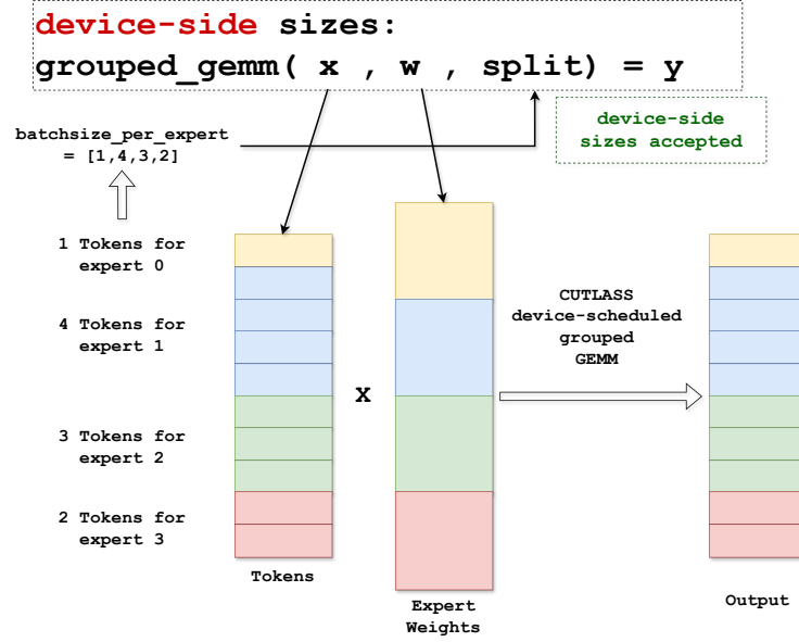
Figure 37 Device-scheduled grouped GEMM executes exact row segments without a host round trip. Device row counts are converted to cumulative offsets. GPU-side preparation then forms the grouped problem list before CUTLASS schedules the compute. The physical buffers retain fixed shapes while the offsets restrict work to the rows assigned to each expert.
