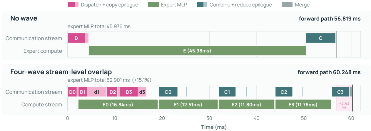
Figure 23 Communication-compute overlap lengthens this measured forward path. This two-node DeepEP v2, EP-MP = 16, 128-expert, top-8 BF16 benchmark uses 16,384 tokens per rank, d = h = 8,192 , and a 32-SM communication budget. Both panels align time to the first dispatch. The four-wave path overlaps communication-stream work with expert computation, but its displayed forward interval is 60.248 ms versus 56.819 ms without waves, a 6.0% increase. Its four expert-compute intervals total 52.901 ms versus 45.976 ms for the single no-wave interval, a 15.1% increase. Durations are manually transcribed from one rank and one measured iteration in the two node-0 Nsight traces. The timeline establishes concurrent execution and component stretch for this instance; it does not identify the contended resource or separate wave granularity from concurrency because no wave-sequential control was archived.
