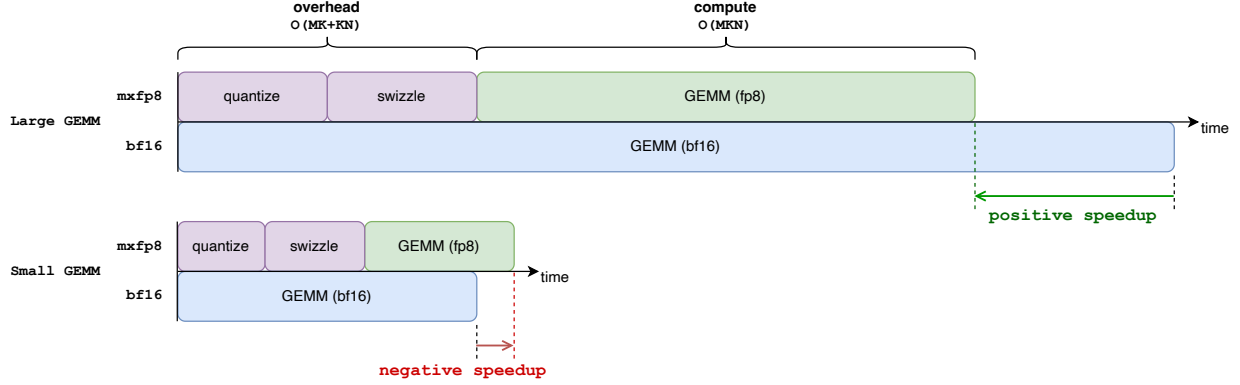
Figure 54 Conversion and layout costs in MXFP8 execution. MXFP8 is faster only when its GEMM savings exceed these costs. This is a schematic cost model, not measured timing. The displayed O(MK + KN) conversion term assumes both operands are quantized on the critical path. In Olmo training, the K \times N weight conversion is normally paid during cache refresh and reused across microbatches, leaving activation conversion as the principal per-invocation cost. For small GEMMs, that remaining overhead can still turn the expected speedup into a slowdown.
