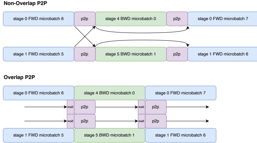
Figure 26 Interleaved-1F1B can overlap P2P communication with independent compute. Without overlap, each stage-boundary transfer is serialized between compute actions. In the steady-state Interleaved-1F1B pattern shown here, both ranks can post their transfers, execute an unrelated virtual-stage action, and defer each wait until the transferred activation or activation gradient is needed. The overlap hides only the portion of P2P time that fits inside this independent compute window.
