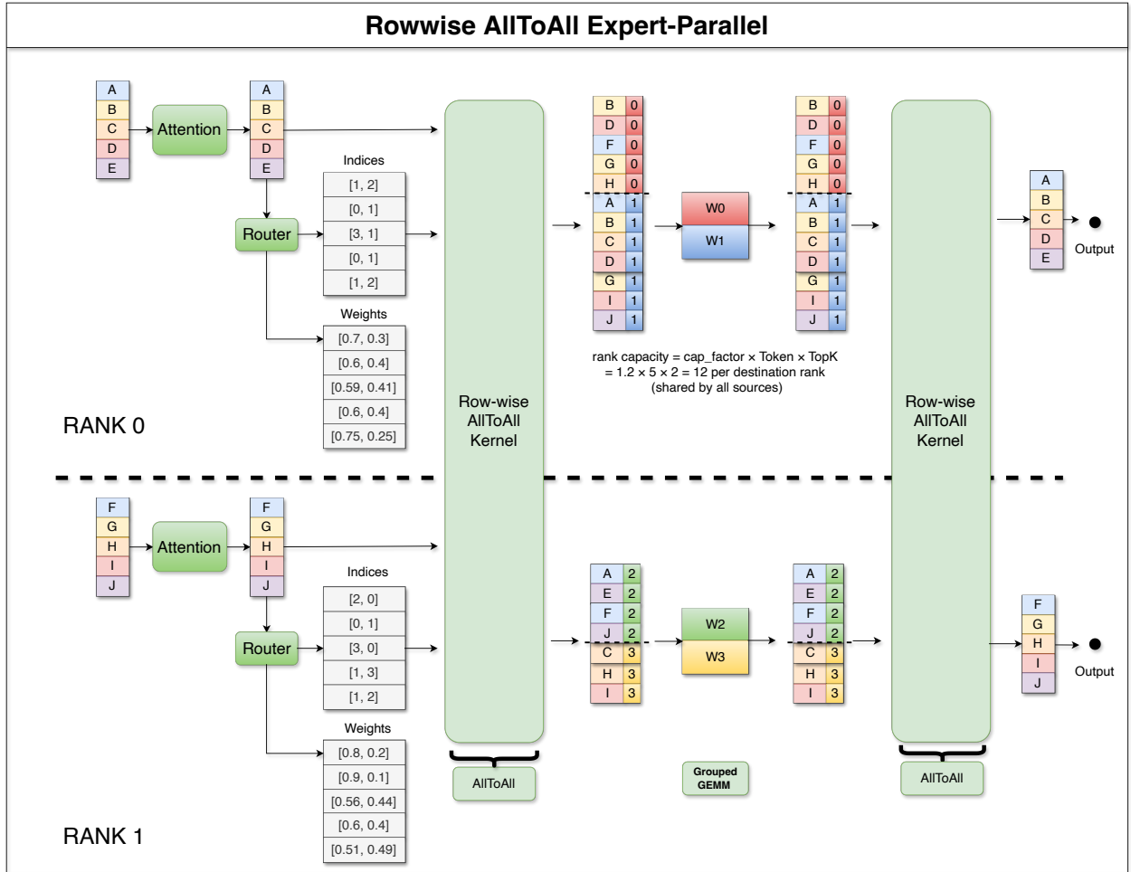
Figure 16 Rowwise EP targets remote expert rows without block packing. In the same illustrative two-rank, top-2 example as Figure 15, GPU-resident route indices drive a rowwise dispatch kernel that places accepted rows directly into fixed-capacity rank- and expert-major storage. Grouped GEMM consumes that layout without a second permutation. Rowwise combine returns expert outputs directly to their source-token positions for weighted merging, without materializing a peer-packed return buffer. The “AllToAll” labels inside the drawing denote the logical rank exchange; the implementation uses indexed one-sided row movement rather than an NCCL all-to-all collective. The drawing explains data layout and movement, not measured performance.
