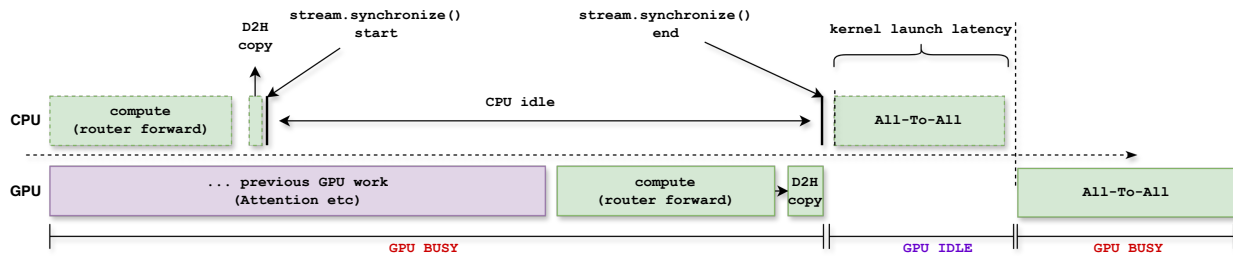
Figure 33 Host-visible split sizes delay the all-to-all launch. The GPU produces route counts, but the synchronized variable-split path must expose them to the CPU before the collective can be launched. If the queue drains at this boundary, the GPU becomes idle until the host receives the counts and submits the all-to-all. The timeline is conceptual and does not encode measured duration.
