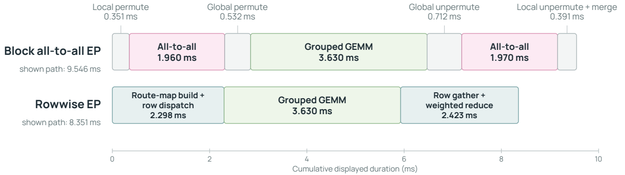
Figure 17 Rowwise EP removes the block-packing stages around expert computation. Block all-to-all EP exposes separate layout and collective stages in dispatch and combine. Each rowwise phase aggregates two displayed subranges: route-map construction plus row dispatch, or row gather plus weighted reduction. Horizontal width shows cumulative displayed duration within each trace, not temporal alignment between traces. The traces were captured on different nodes, so this is mechanism evidence rather than a controlled performance comparison.
