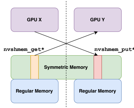
Figure 18 Symmetric memory makes matching offsets remotely addressable. Participating EP-MP ranks create corresponding heap regions. A local offset and a peer-rank index therefore identify the matching remote location, allowing a GPU kernel to address an expert-capacity row directly. The allocation establishes addressability; ordering and buffer-reuse rules still determine when a row may be read or overwritten.
