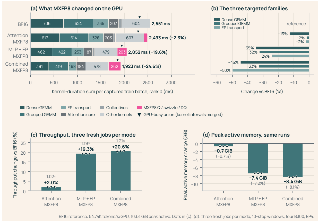
Figure 59 Kernel-time breakdown, throughput, and memory across the four MXFP8 modes. The combined recipe reduces the rank-0 kernel-duration sum by a quarter. Panels (a,b) use profiled kernel durations to identify changed work; panel (c) uses unprofiled runs for throughput because tracing perturbs the launch-heavy combined path. (a) Kernel-duration sums per captured train batch on rank 0 by kernel family, means of three captured batches per mode. Teal families are the ones MXFP8 targets, gray families are not targeted, and pink is the added quantization, scale-swizzle, and dequantization work (75.5, 203.1, and 262.1 ms per batch; 3.0%, 8.0%, and 10.3% of the BF16 sum). Family sums overlap across streams and are not an additive wall-time model; the triangle marks the union of kernel-busy intervals, which shrinks by 1.3%, 16.3%, and 20.2%. (b) Change of the three targeted families relative to BF16; the bars in each row are, top to bottom, dense GEMM, grouped GEMM, and EP transport, in the colors of (a). The EP-transport family includes barrier kernels; the payload-moving kernels alone fall by 41% in both the MLP+EP and combined modes, so part of the combined -50% is reduced waiting. (c) Throughput change over three fresh distributed jobs per mode; bars are means of the three ten-step windows and dots are the repetitions. The BF16 reference is 54.74K tokens/s/GPU and the largest sample standard deviation is 0.14K, smaller than the dot markers. (d) Peak active memory change in the same runs from the 103.40 GiB BF16 reference. Four B300 GPUs, EP = 4, uniform routing, and identical initialized weights, inputs, and routing in every mode (Table 26); these are systems measurements at one operating point, not training-quality evidence (Section 11.3.5).
