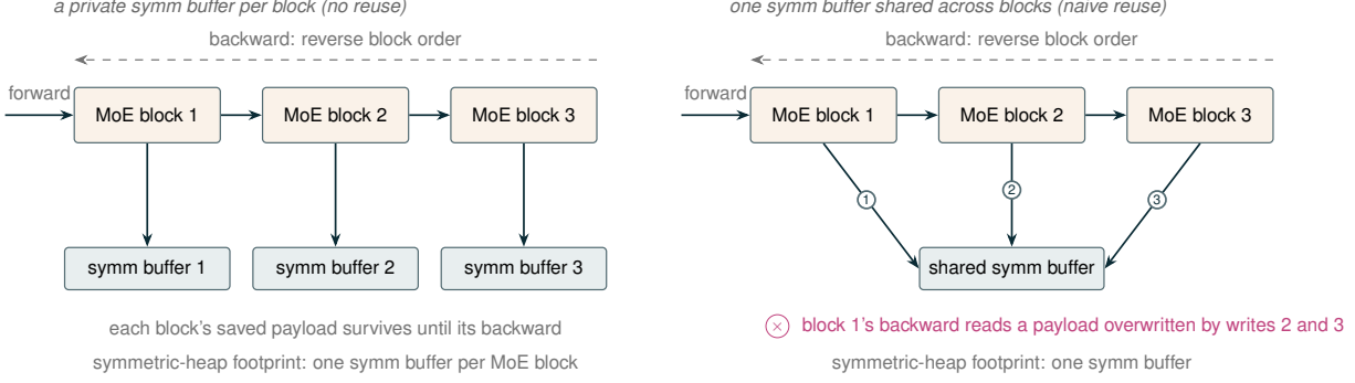
Figure 21 A shared symmetric buffer saves memory but can overwrite saved payloads. With a private symmetric buffer per block, each saved payload survives untouched until its block’s backward, but resident symmetric memory grows with the number of local blocks; one shared buffer keeps the footprint constant, but forward visits blocks in order 1, 2, 3 while backward returns in order 3, 2, 1, so block 1’s backward reads a payload that later blocks have overwritten. Scratch buffers, which no later operation reads, safely take the shared path; payloads saved for backward keep per-block slots whose reuse is controlled by the lease system of Figure 22, and activation recomputation turns a saved payload back into scratch, restoring the shared option. Conceptual illustration with no measured quantities.
