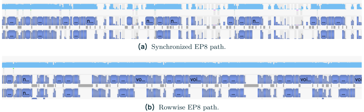
Figure 75 Magnified GPU kernel rows of the two captures. Each strip crops the CUDA HW utilization band and its two All-Streams kernel rows from the corresponding panel of Figure 74, over an equal-width sub-window of each timeline. In the synchronized capture (a), the utilization band is repeatedly interrupted and the kernel rows show recurring idle gaps where the device waits for host submission. In the rowwise capture (b), the band is continuous and the kernel rows are densely packed. The two strips come from separate runs whose timeline zoom levels differ, so bar widths are not comparable across panels; the crops illustrate the submission mechanism, not a throughput measurement.
