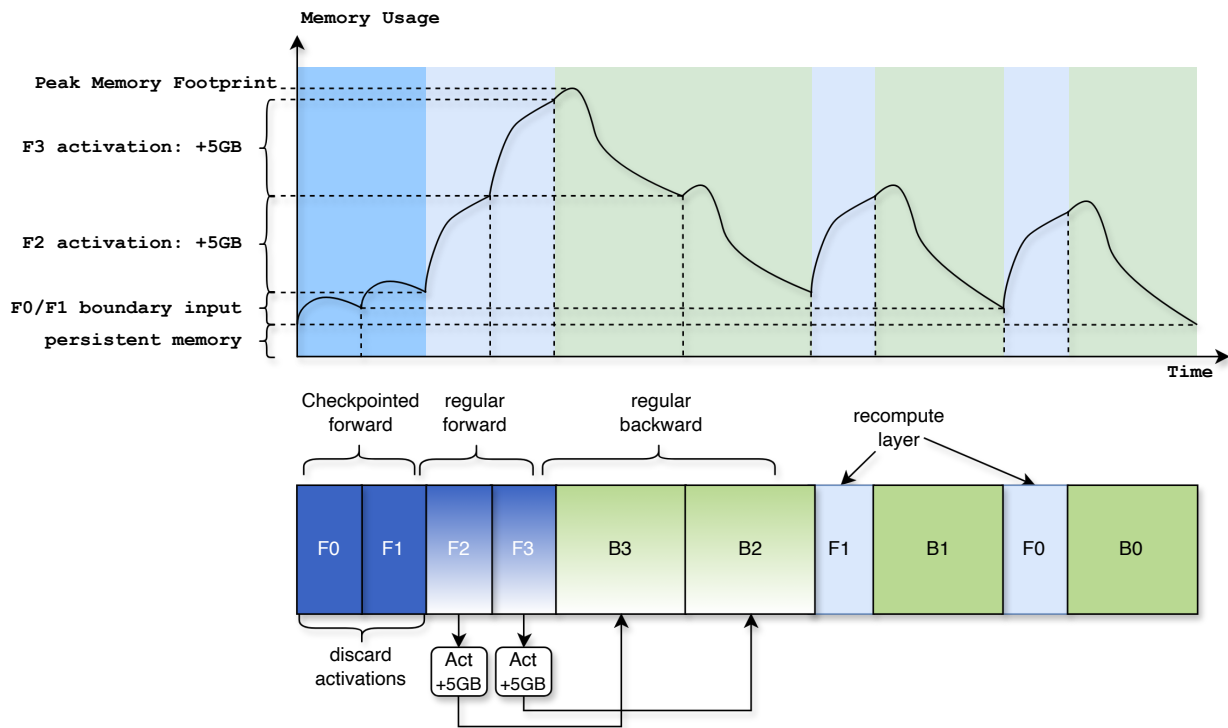
Figure 60 Layer recompute trades additional forward work for lower activation memory. In this illustrative schedule, F0 and F1 are checkpointed, whereas F2 and F3 retain their backward-needed activations. Checkpointing discards F0/F1’s internal activations but retains their boundary inputs; the two forwards are therefore recomputed immediately before B1 and B0. The 5 GB increments and smooth memory curve illustrate the accounting and are not measurements from a training run.
