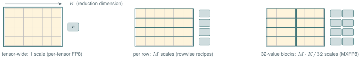
Figure 53 Scale granularity is a spectrum along the reduction dimension. One tensor-wide scale must cover the largest value in the tensor, per-row scales track variation more closely, and 32-value block scales track it most tightly at the highest metadata cost. Conceptual illustration with no measured quantities.
