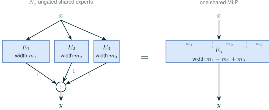
Figure 68 Combining ungated shared experts into one wider MLP. Every token reaches all N_s shared experts, and their outputs are added with fixed unit coefficients, so the sum equals one MLP whose intermediate width is the sum of the branch widths (Equation 76). The dashed marks show where each original partition sits after concatenating the up and gate projections and stacking the down projections; box widths are drawn proportional to intermediate widths.
