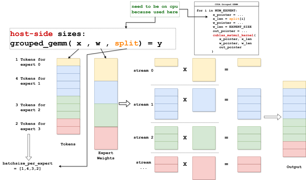
Figure 36 A host loop executes exact-size expert GEMMs. It avoids padded arithmetic, but GPU-produced row counts must become host-visible before the runtime can submit the per-expert operations. The separate streams in this conceptual drawing are not required by the method; the legacy Olmo fallback submits its GEMMs on the current stream.
