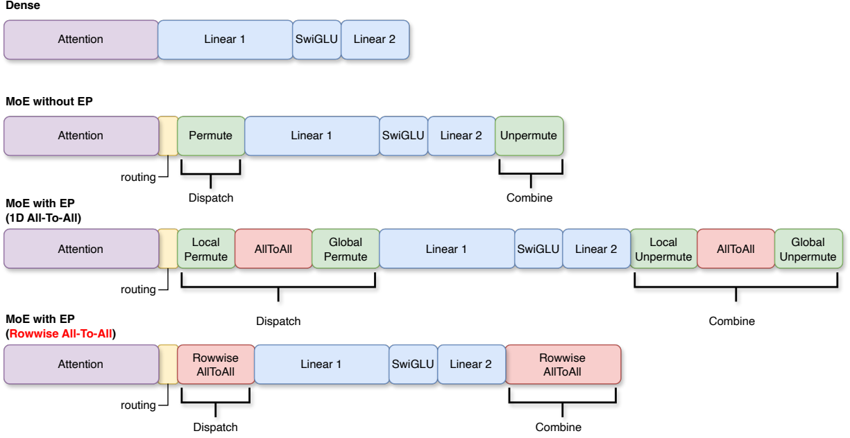
Figure 14 Routing overhead grows from dense execution to local MoE and conventional all-to-all EP. A dense MLP has no routing path. MoE without EP adds one local permutation into expert order and one unpermutation back to token order. Conventional all-to-all EP expands dispatch into permute–all-to-all–permute and combine into unpermute–all-to-all–unpermute. Rowwise EP instead attempts to move selected rows directly between token-source and expert ranks. The drawing is not performance evidence.
