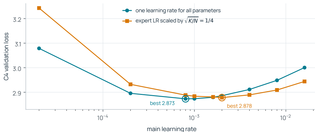
Figure 67 Sparsity-scaled expert learning rates did not improve the tested sweep. Each point is one 0.43B@2.51B, top-4-of-64 MoE trained for 150B tokens. The teal sweep uses one learning rate for all parameters; the orange sweep sets \eta_{\text{expert}} = \eta_{\text{main}} \sqrt{K/N} = \eta_{\text{main}}/4 . Both sweeps cover the same nine main learning rates; markers are observed runs and connecting lines are visual guides. After independently tuning the main learning rate, the best unscaled run reaches C4 (Raffel et al., 2020) validation loss 2.873 at 8 \times 10^{-4} , while the best sparsity-scaled run reaches 2.878 at 2 \times 10^{-3} . Each point is a single run without seed replication, so the comparison is directional rather than a precise estimate of the gap.
