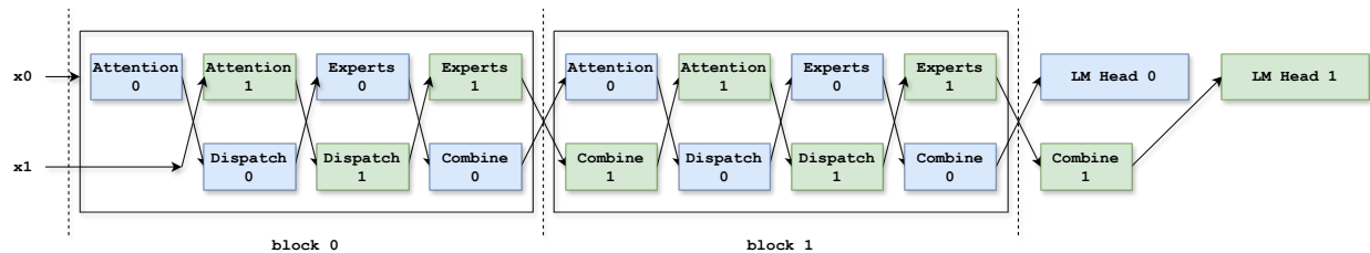
Figure 63 Two-batch overlap interleaves two half-microbatch lanes across adjacent MoE blocks. Blue and green denote lanes 0 and 1. The schedule interleaves attention, expert computation, and expert-parallel dispatch and combine so that communication from one lane can run alongside computation from the other. The arrows show data dependencies; the visual overlap alone does not imply a wall-time speedup.
