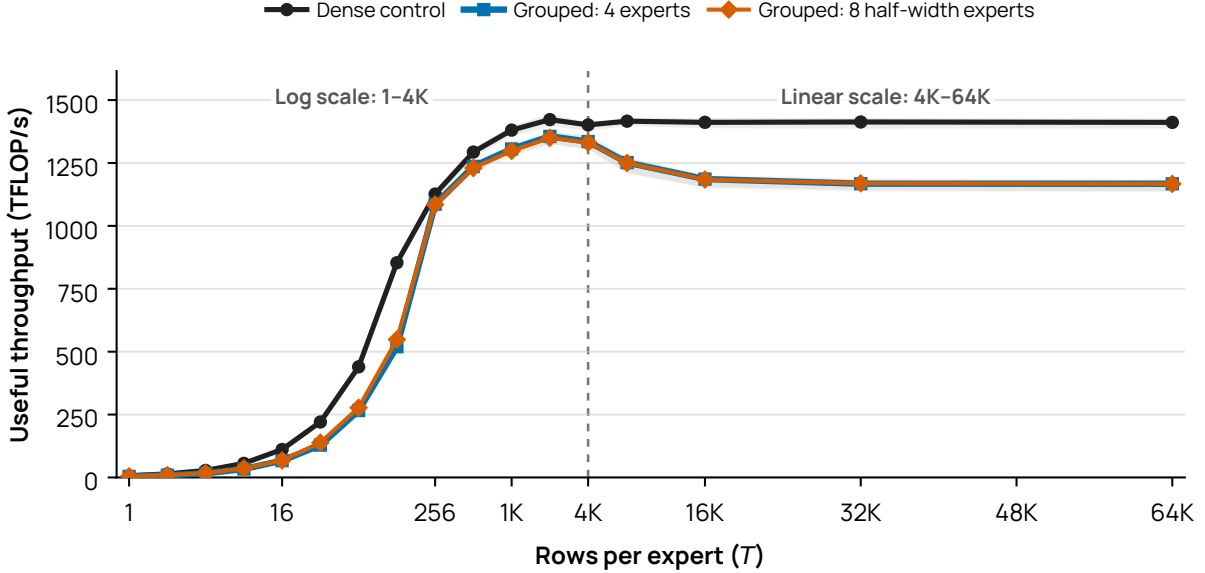
Figure 39 Splitting one projection into four or eight expert GEMMs. The four-expert path executes four [T, 8192] @ [8192, 20480] GEMMs; the eight-expert path executes eight [T, 8192] @ [8192, 10240] GEMMs. Both are exact partitions of the same [T, 8192] @ [8192, 81920] dense projection and therefore match its useful FLOPs, weights, and outputs. Grouped inputs repeat the dense input four or eight times. Curves show means across eight paired trials, one on each of eight B300 GPUs, and light bands show the full eight-GPU ranges; each GPU measures the dense control with both grouped partitions, and its two dense measurements are averaged before the dense curve is summarized. The horizontal axis is logarithmic through T = 4096 and linear thereafter; the dashed divider marks the scale change, and no values are omitted. The final two points, T = 32,768 and 65,536 , are oversized diagnostics rather than representative training shapes. Only the projection is timed; Appendix A.11 records the complete timing protocol and representative ratios.
