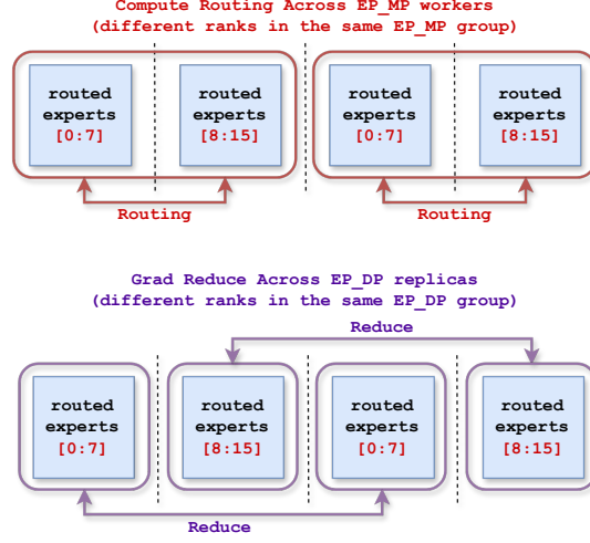
Figure 13 EP-MP routes tokens; EP-DP reduces gradients. Within each EP-MP group, different ranks hold different expert shards, so routed token rows move between those ranks for expert computation. Within each EP-DP group, ranks holding replicas of the same expert shard reduce that shard’s gradients together: experts 0–7 reduce with their replicas, and experts 8–15 reduce with theirs. Token communication and gradient reduction therefore use different rank groups.
