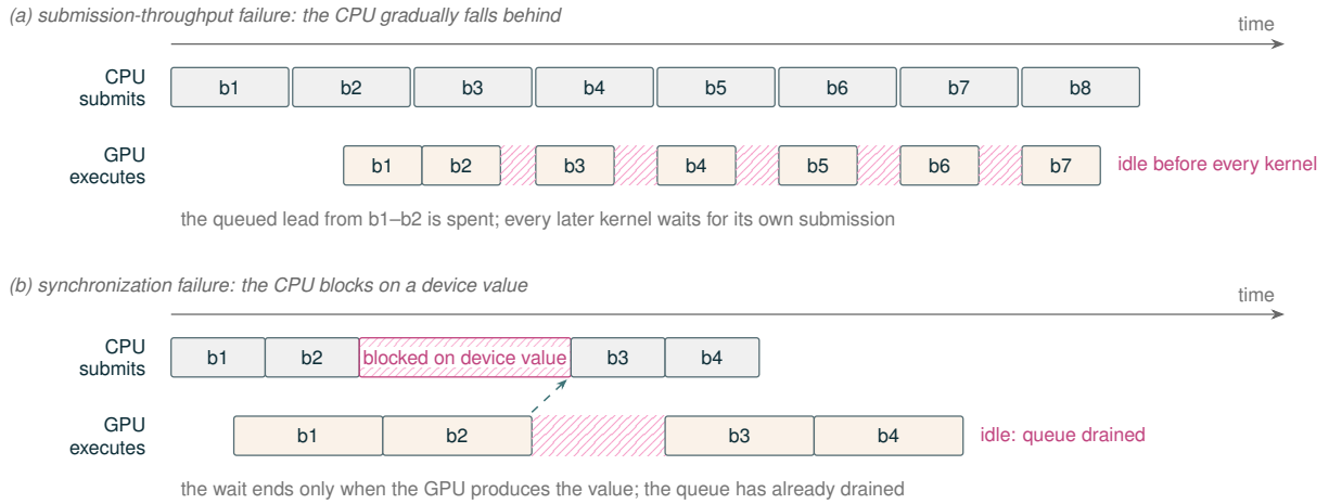
Figure 29 GPU idle intervals caused by slow submission and host waits. (a) When submitting a block costs the CPU more time than executing it costs the GPU, the queued lead is spent and every later kernel waits for its own submission; the GPU idles a little before every block. (b) When the CPU blocks on a device value, submission stops entirely: the GPU finishes the queued work, sits idle until the value is produced and the host resumes, and the host must then rebuild its lead. Conceptual illustration with no measured quantities.
