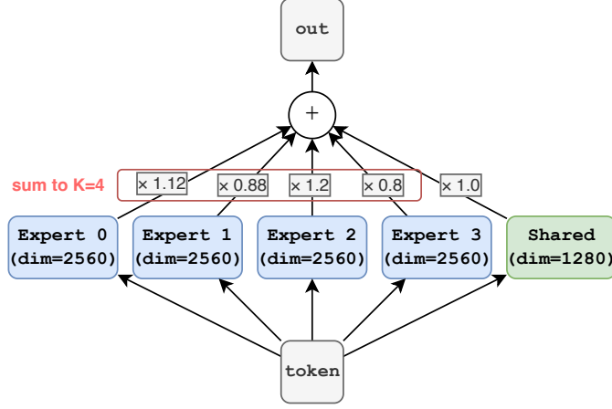
Figure 69 Merging four routed-expert outputs with one shared-expert output. In the Olmo rule, selected routed coefficients vary by token but sum to K = 4 , so their mean is one; the shared-expert coefficient is also one. Routed and shared experts may have different intermediate widths because every branch returns a model-width tensor before the addition. Conceptual illustration with no measured quantities.
