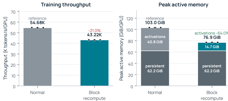
Figure 62 Block recompute removes nearly two thirds of activation memory at a one-fifth throughput cost in this matched configuration. Bars show the arithmetic mean of three fresh-process repetitions; dots show the individual ten-step windows, and the sample standard deviations are smaller than the dot markers. Normal training in this campaign sustains 54.68K tokens/s/GPU at 103.03 GiB peak active memory; recomputing every transformer block sustains 43.22K tokens/s/GPU at 76.90 GiB, 20.95% lower throughput for 26.13 GiB (25.36%) less peak memory. The lower segment of each memory bar, labeled “persistent”, is the memory resident between steps (parameters, gradient buffers, optimizer states, and persistent buffers), 62.21 GiB in both modes; the reduction therefore falls entirely on the transient activation part, which shrinks from 40.82 to 14.69 GiB. Measurements use four NVIDIA B300 GPUs and the fixed model, batch, routing, and timing protocol described in the text.
