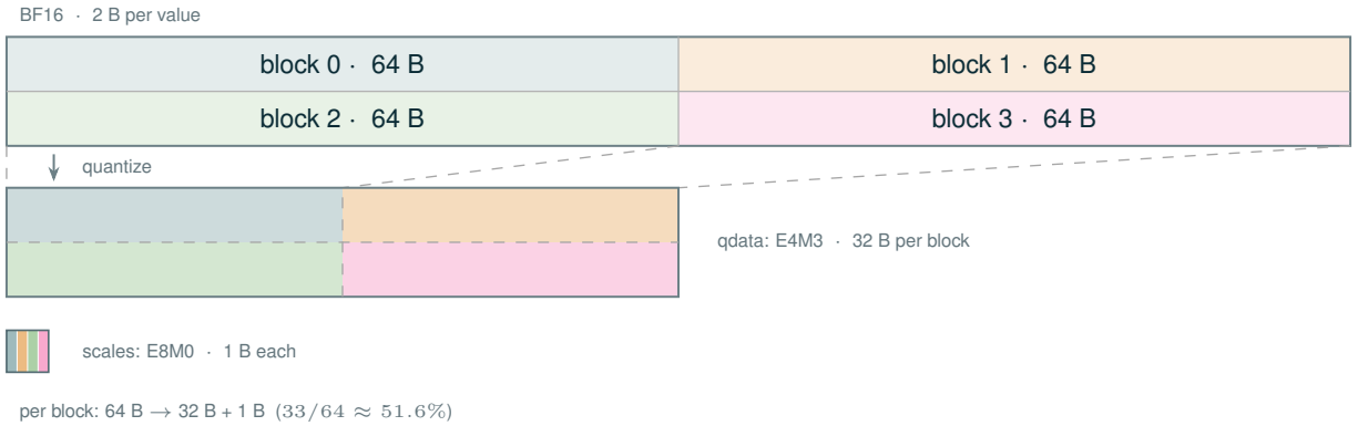
Figure 51 Quantization produces one contiguous qdata array and one contiguous scale array. Sizes are drawn to byte scale for a two-row tensor with two 32-value blocks per row: each 64-byte BF16 block becomes a 32-byte E4M3 qdata block, half as wide, and the flattened scale array adds one E8M0 byte per block, each scale 1/32 the width of a qdata block. The four scales are the narrow strip at the lower left, drawn at true width; color marks which block each scale covers, and the dashed spans are logical: neither array is fragmented. Conceptual illustration with no measured quantities.
