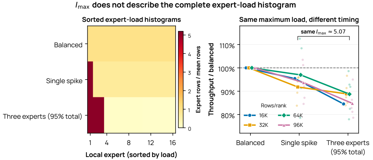
Figure 72 The same I_{\max} can describe different grouped GEMM workloads. Left: sorted expert loads for a representative 64K-row case. Right: rank-local grouped GEMM throughput normalized to the balanced assignment in the same process. Large markers report arithmetic means, while small translucent points show five independent runs on the same B300. In each run, let a be the base expert index. The matched single spike overloads expert a , while the three-hot assignment overloads experts (a, a + 5, a + 10) \bmod 16 ; the five values of a are 0, 3, 6, 9, and 12. Every run averages 20 queued CUDA-event samples after 10 warm-ups. The benchmark isolates one BF16 d = h = 4096 projection and excludes dispatch, communication, and cross-rank waiting.
