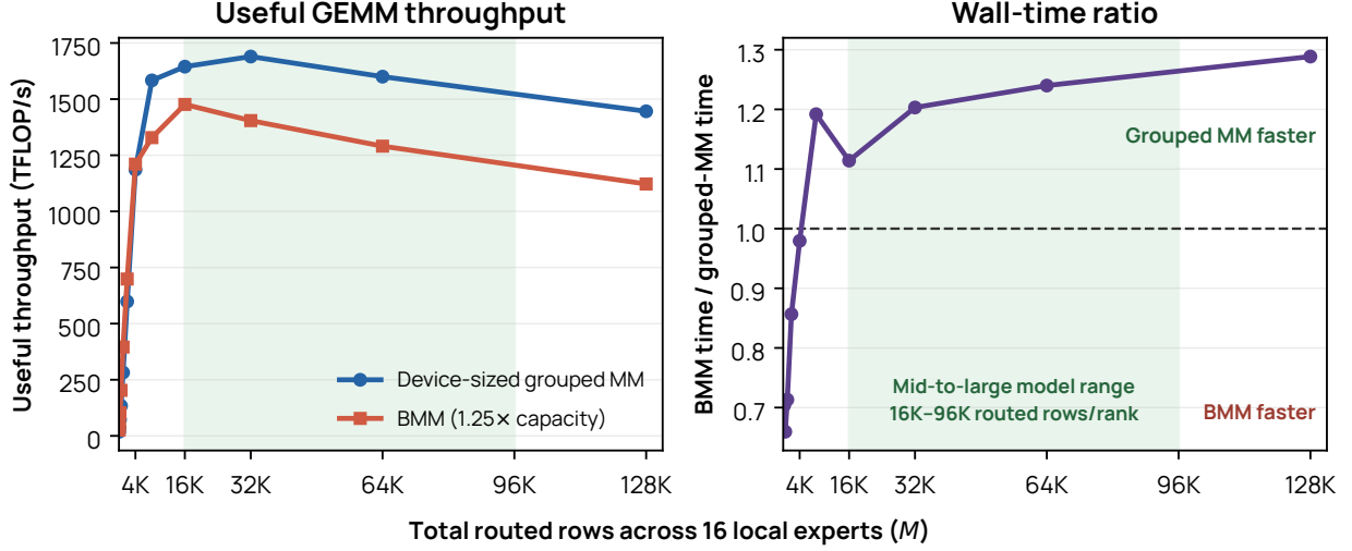
Figure 38 Grouped GEMM and capacity-padded BMM across routed-row counts. Grouped GEMM is faster throughout the shaded mid-to-large-model range. The experiment isolates one BF16 square expert projection on one B300 with N_{\text{local}} = 16 and d = h = 4096 . The horizontal axis is total routed rows across the 16 local experts; routed rows count expert rows, not unique input tokens, since each token contributes one row to each of its top- K experts, and balanced routing gives M/16 valid rows per expert. The green band marks the representative 16K–96K rank-local operating range. Its endpoints summarize variation in microbatch and routing choices rather than one fixed microbatch size, sequence length, top- K , or local-expert count; Appendix Table 42 gives concrete configurations. BMM reserves exactly 1.25\times capacity per expert, while grouped GEMM executes only valid rows. Left: useful throughput counts only valid-row FLOPs. Right: values above one indicate that grouped GEMM is faster. Each point is the mean of 20 queued CUDA-event samples after 10 warm-ups; all timed operations are submitted behind one device-side gate and released only after the host has queued the complete batch, so small shapes are not dominated by Python launch gaps.
