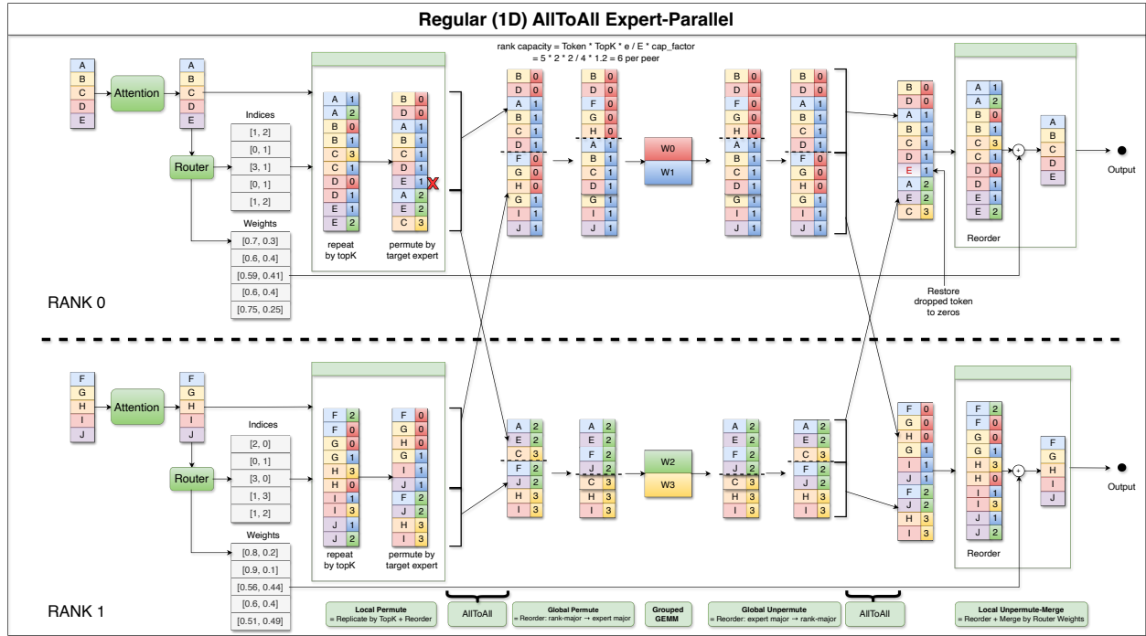
Figure 15 Block all-to-all EP exposes the complete packing path. In this illustrative two-rank, top-2 example, local dispatch replicates token rows and packs routes by destination rank. The first all-to-all exchanges peer-contiguous blocks, and a global permutation converts the received rank-major layout into local-expert order for grouped GEMM. Combine reverses the global layout conversion and all-to-all, restores token order, fills a capacity-dropped route with zero, and merges route contributions using the router weights. The drawing explains data layout and movement, not measured performance.
