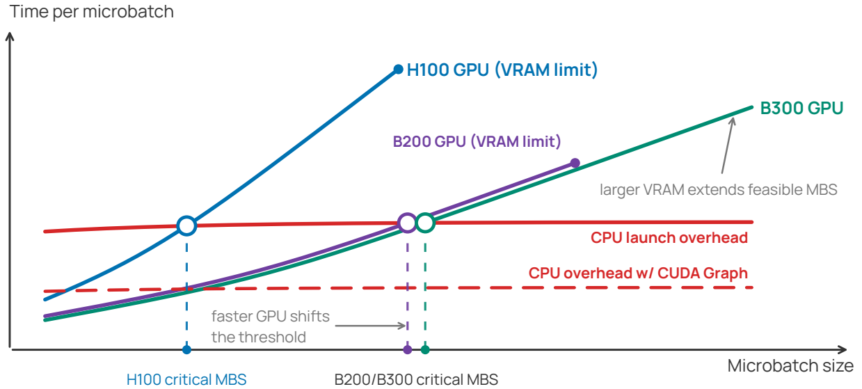
Figure 32 A faster GPU can move the critical microbatch size to the right. The solid red curve represents CPU submission time, while the blue, purple, and green curves represent H100, B200, and B300 execution time. Below a crossover, the device can consume work faster than the host supplies it; faster execution with an unchanged host path therefore requires a larger microbatch to restore submission headroom. Additional GPU memory can extend the feasible microbatch range, while reducing submission overhead (dashed red; CUDA Graph replay is one way to reduce this overhead) can move the crossover to the left. The curves, intersections, and memory limits are qualitative annotations rather than measurements; no numerical critical size is implied.
