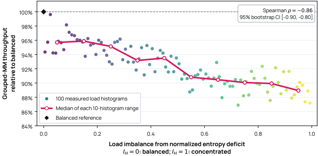
Figure 40 Grouped GEMM throughput generally falls as expert loads concentrate. The experiment isolates one BF16 square expert projection on one B300 with N_{\text{local}} = 16 , M = 65,536 routed rows, and d = h = 4096 . We draw symmetric-Dirichlet proposals, convert them to exact eight-row-aligned counts with at least one tile per expert, and select ten distinct histograms from each of ten equal-width I_H ranges. Every dot therefore has the same total rows, operands, dimensions, and useful FLOPs. Each dot averages four fixed expert-index permutations in each of three fresh processes. Each of those 12 conditions averages 20 queued CUDA-event samples after 10 warm-ups; execution order is randomized and balanced controls bracket every ten cases. The magenta curve connects the median of each ten-histogram range. The correlation and bootstrap interval are computed over the 100 histogram means. This kernel-only test excludes dispatch, communication, and cross-rank waiting.
