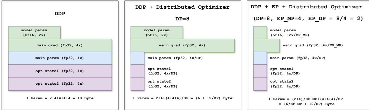
Figure 9 The distributed optimizer and EP reduce different parts of DDP’s persistent parameter-sized training state. Under the illustrated BF16-execution, FP32-gradient, and two-moment FP32 optimizer policy, naive DDP uses 18 bytes per parameter. Sharding the FP32 main weights and optimizer states evenly over D replica ranks reduces this to 6 + 12/D bytes while compute weights and gradient buffers remain replicated. Sharding routed-expert compute weights and gradients over the expert-parallel model-sharding degree M_E (EP-MP; defined in Section 5) further reduces their per-rank memory contribution to 6/M_E + 12/D bytes when D = M_E D_E . Dense and shared parameters follow their separate replica groups. This accounting excludes execution working memory, including activations, routing and communication buffers, kernel workspaces, execution caches, and allocator fragmentation, as well as uneven shards and small auxiliary tensors that are not sharded.
