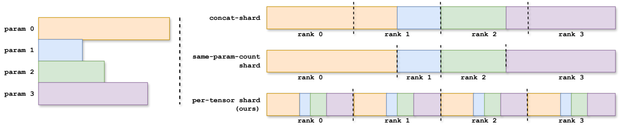
Figure 10 Optimizer-state layout choices. Colors identify eligible FP32 optimizer-state tensors associated with different model parameters; they do not represent the replicated BF16 compute weights. Dashed lines mark the ranges assigned to each rank in an optimizer replica group of size D = 4 . Concatenate-then-shard balances the flattened optimizer state globally but requires explicit view and offset metadata. The same-param-count baseline preserves whole tensors but can severely imbalance bytes. Olmo instead divides each eligible main-weight and optimizer-state tensor independently into D equal contiguous shards.
