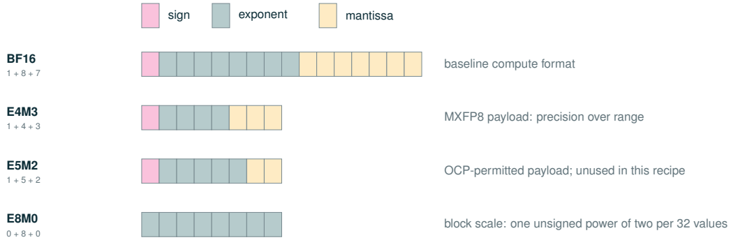
Figure 49 Bit layouts of the baseline, payload, and scale formats. BF16 keeps eight exponent bits and seven mantissa bits. The E4M3 payload trades exponent range for mantissa precision; E5M2 makes the opposite trade and is permitted by OCP MX but unused in the Olmo recipe. The E8M0 scale is an exponent-only format: one unsigned power of two per 32-value block, with no sign and no mantissa.
