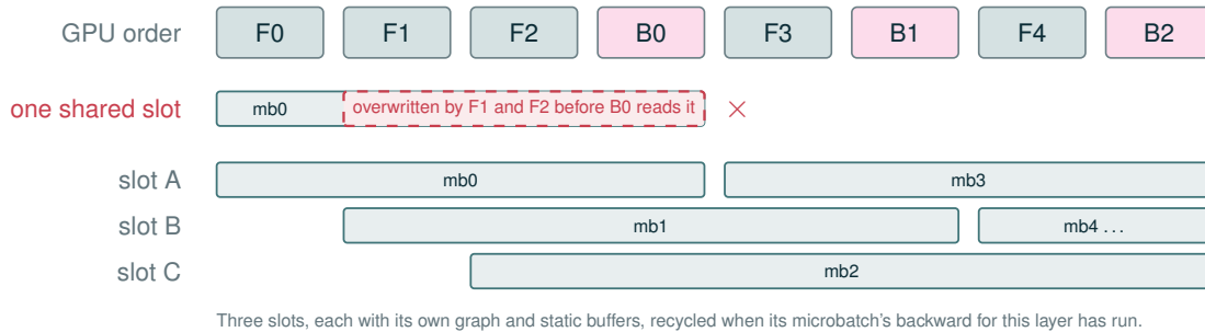
Figure 65 Under a pipeline schedule, static per-layer replay needs one saved-context slot per in-flight microbatch. (a) Without a pipeline the backward of each microbatch consumes the layer’s saved context before the next forward overwrites it, so one graph per layer serves every microbatch. (b) With three microbatches in flight, a shared slot is overwritten by F1 and F2 before B0 reads it; three slots, each with its own graph and static buffers, are recycled as each microbatch’s backward for the layer completes. Conceptual illustration after the design described for Megatron-Core (Yan et al., 2026); no measured quantities.
