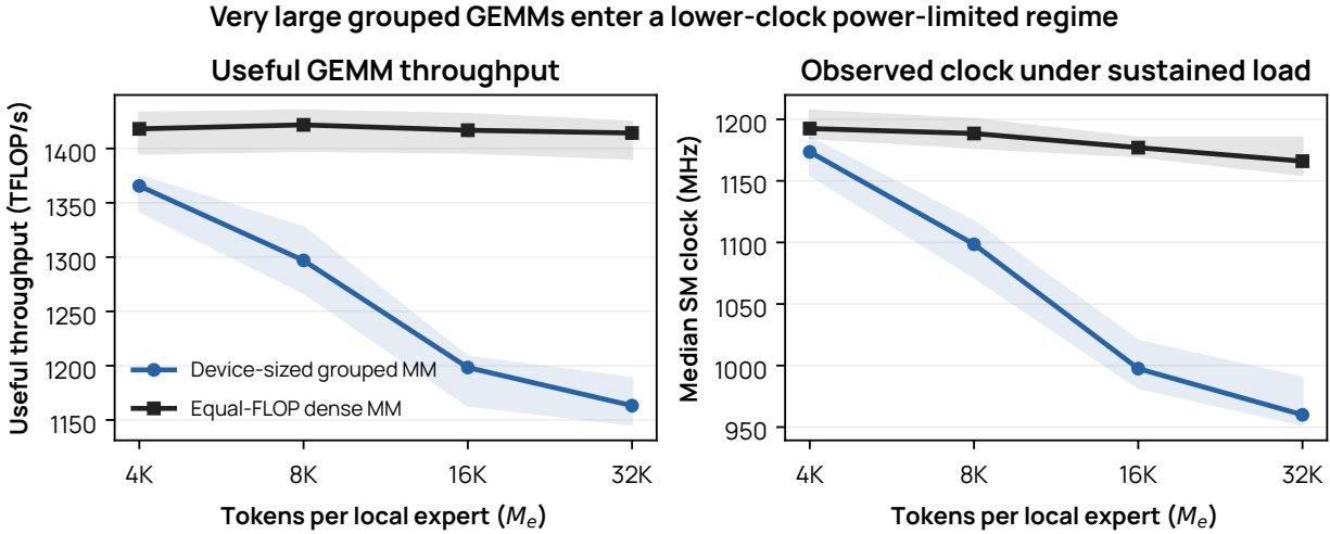
Figure 73 The very-large- M_e grouped GEMM slowdown follows SM clock, not per-clock efficiency. Lines show medians and bands show the full range across eight trials. Both paths execute the same useful FLOPs, although the dense control reuses one weight matrix while grouped GEMM reads 16 expert matrices. The software power-cap limiter was active in 99.3% of telemetry samples; no thermal, hardware-brake, or reliability limiter was observed.
