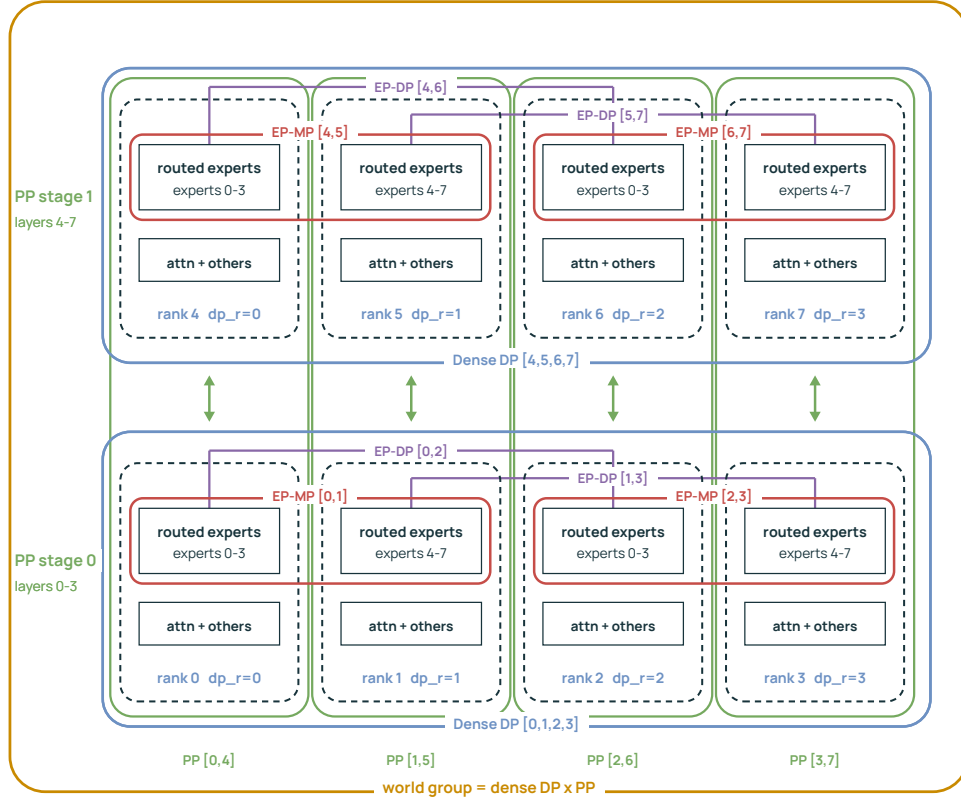
Figure 28 The same ranks participate in several logical topologies. This illustrative eight-rank example uses PP = 2 , DP = 4 , EP-MP = 2 , and EP-DP = 2 . Each PP stage stores one layer range; EP-MP pairs form a complete expert set; EP-DP pairs connect replicas of an expert shard; and PP groups join matching data-parallel coordinates across stages. Context parallelism is omitted. The diagram establishes group membership, not the hardware path or a measured production placement.
